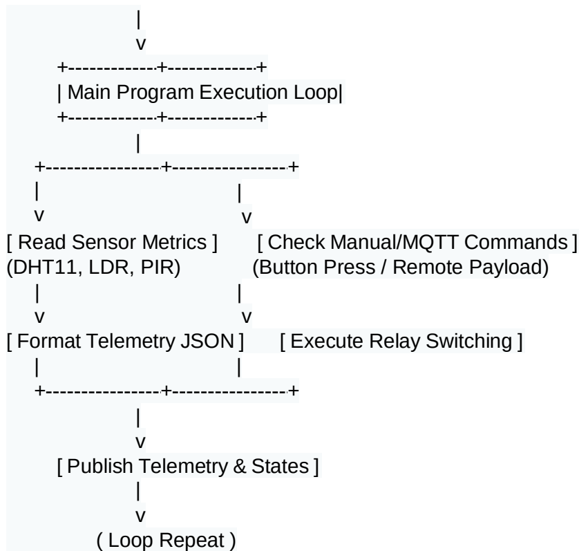
Figure 5.3: Firmware Execution State Flowchart
