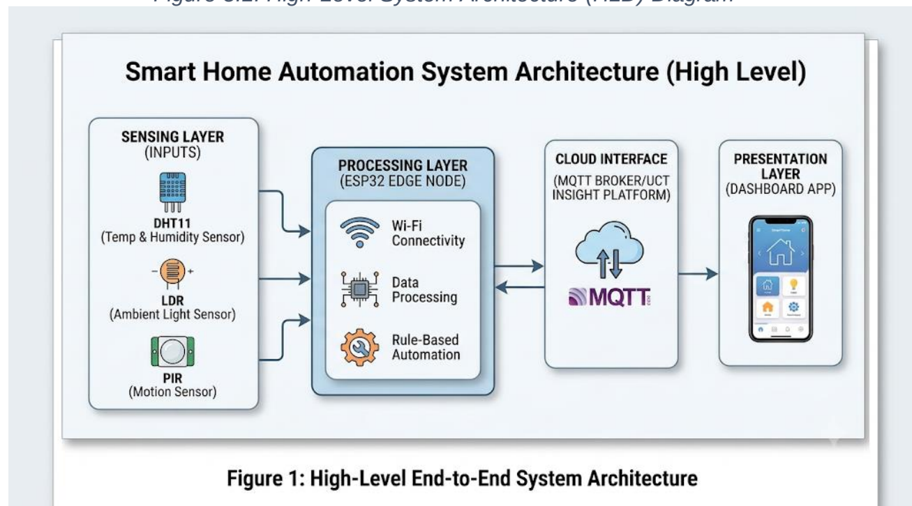
Figure 5.1: High-Level System Architecture (HLD) Diagram
